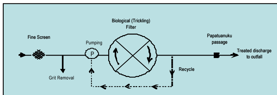
Figure 1: A schematic showing the unique BTF arrangement for Hastings
