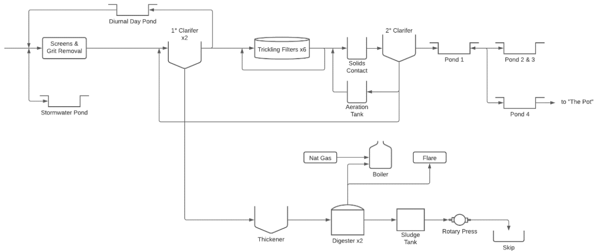
Figure 2: Levin WWTP, Existing Process
