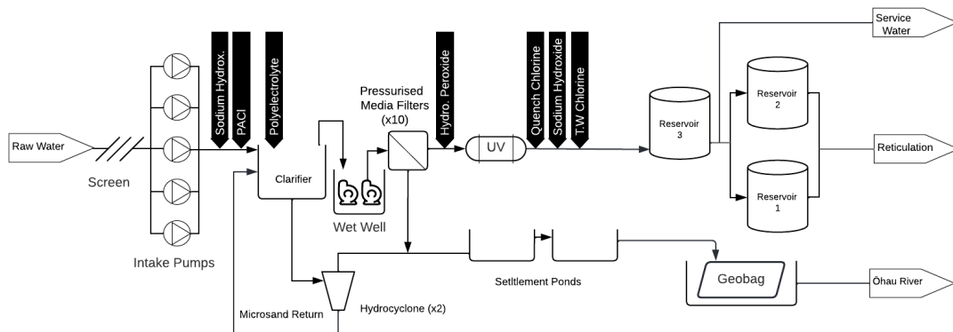
Figure 4: Levin WTP, Existing Process
