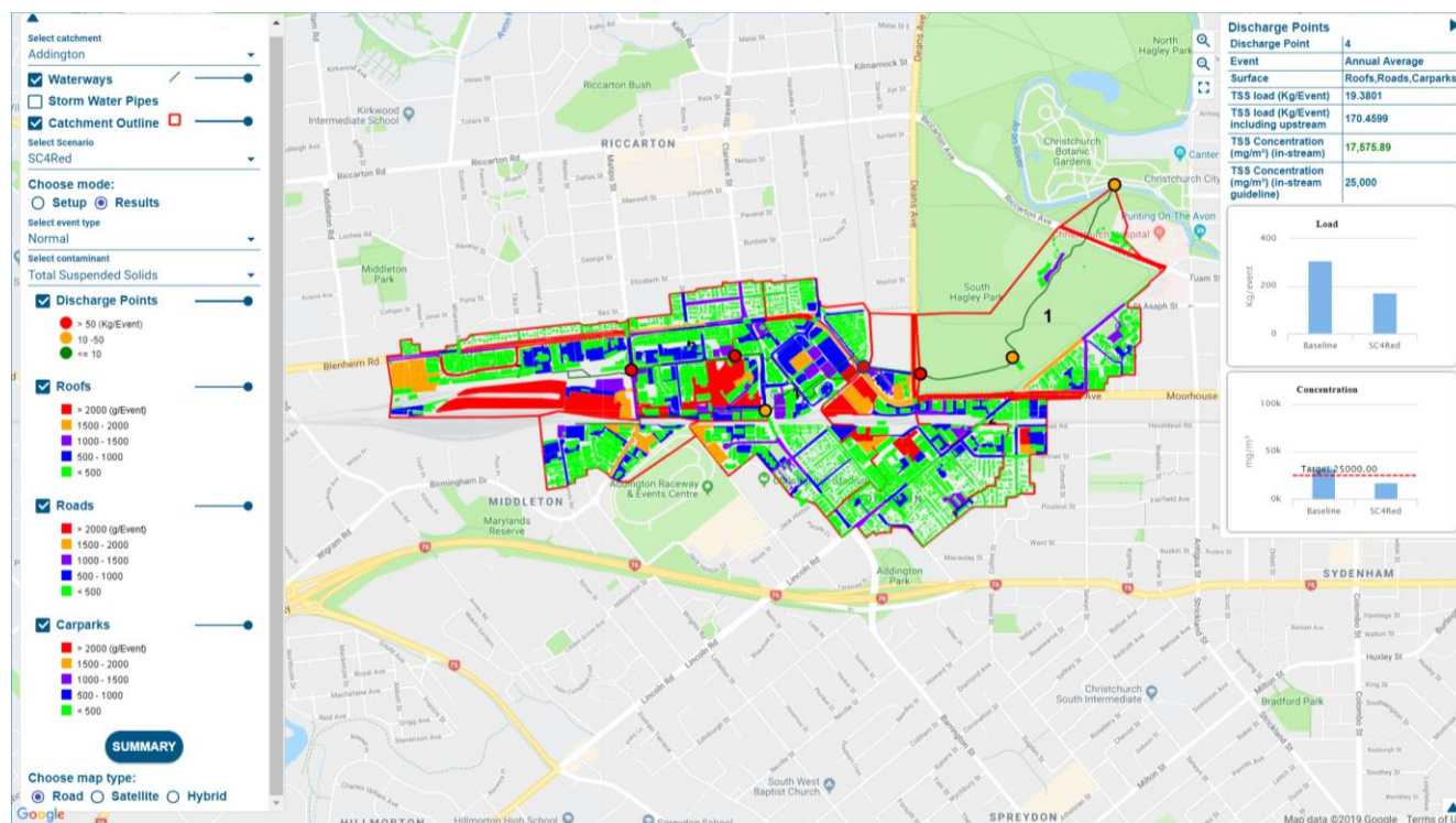
Figure 6: Mitigation Scenario - Load reduction at Sub-Catchments 4 and 7
