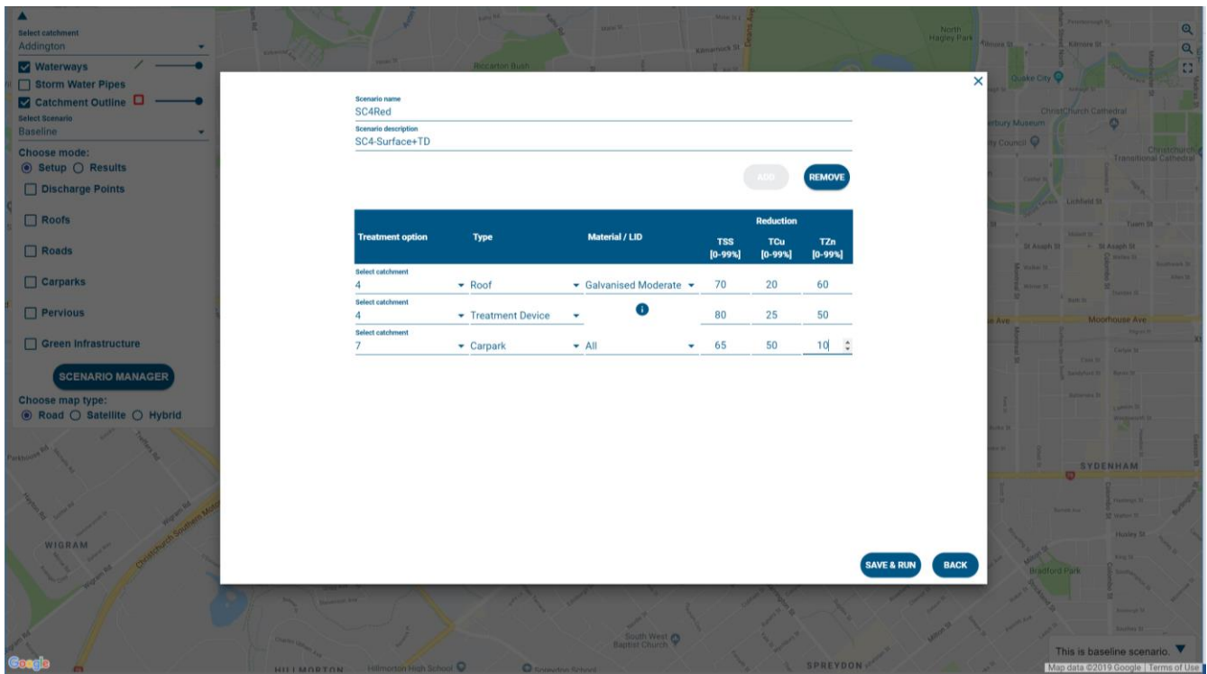
Figure 5: Scenario Generation – Load Reduction through source control and Treatment Devices
