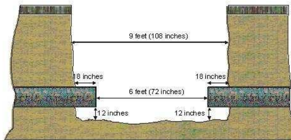
Figure 4: Access pit – side view
