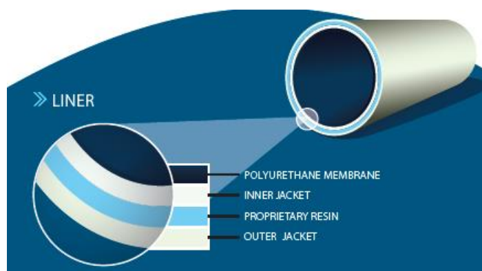
Figure 1: Liner details
