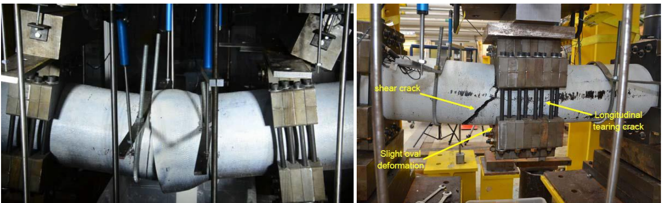
Figure 25 & 26 Rotational Joint testing of and Shear Testing Aquapipe lined pipe
