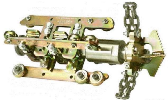
Figure 10: Cleaning Head
