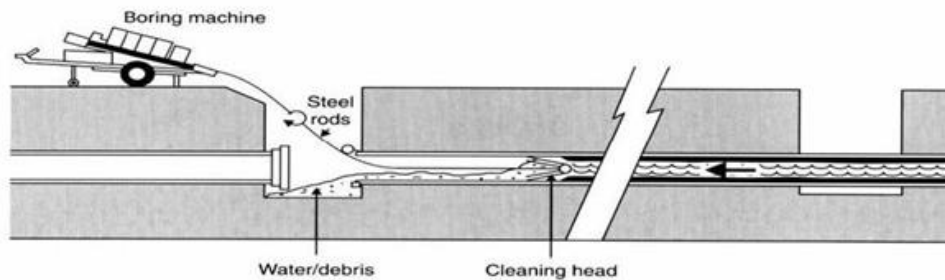
Figure 8: Pipe Cleaning
