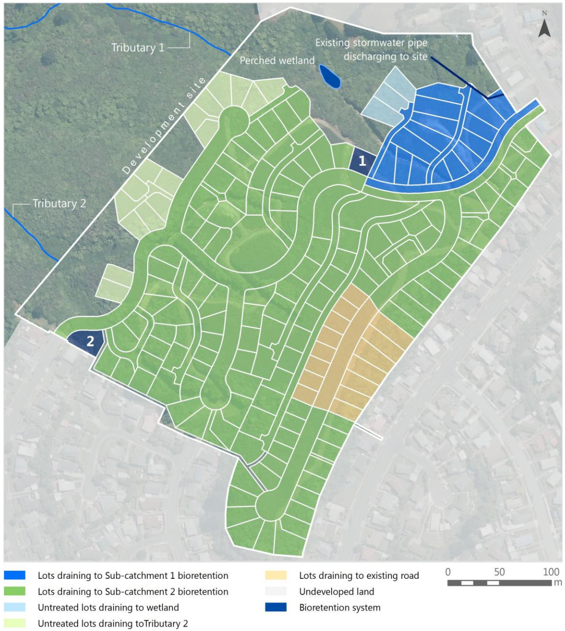
Figure 3: Post-development catchments and treatment locations
