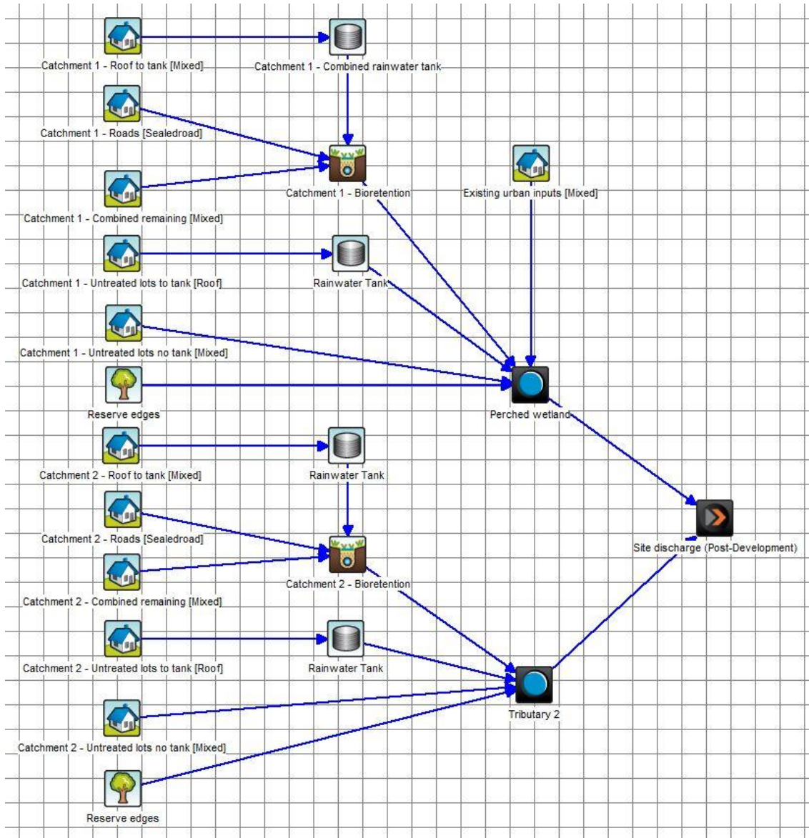
Figure 4: MUSIC structure for the post-development condition with integrated stormwater management
