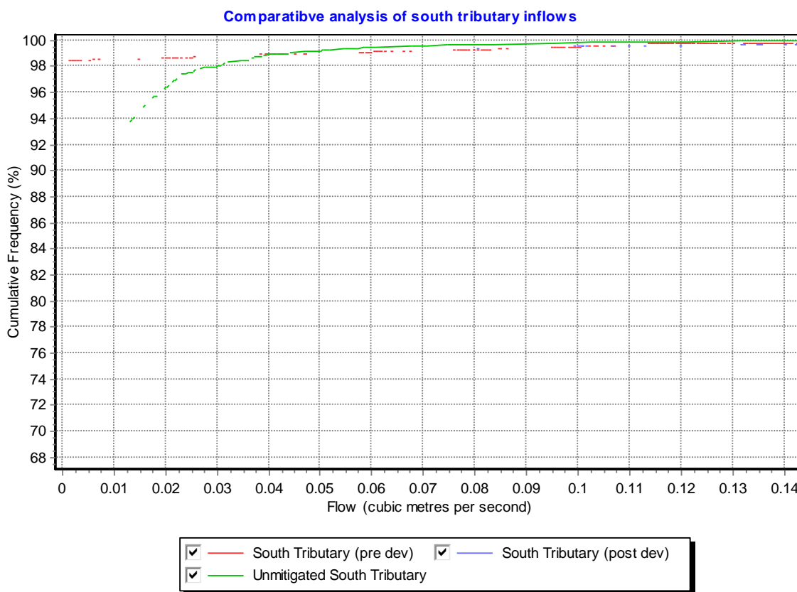
Figure 6: Cumulative frequency plot of discharge to Tributary 2
