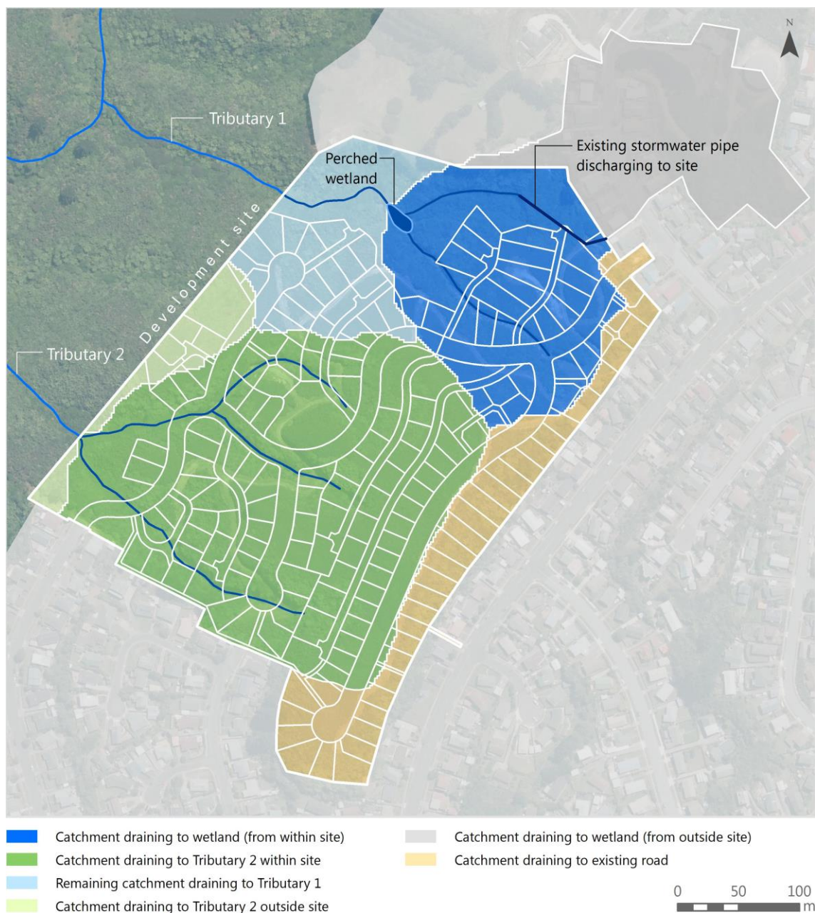
Figure 1: Pre-development catchments and drainage patterns
