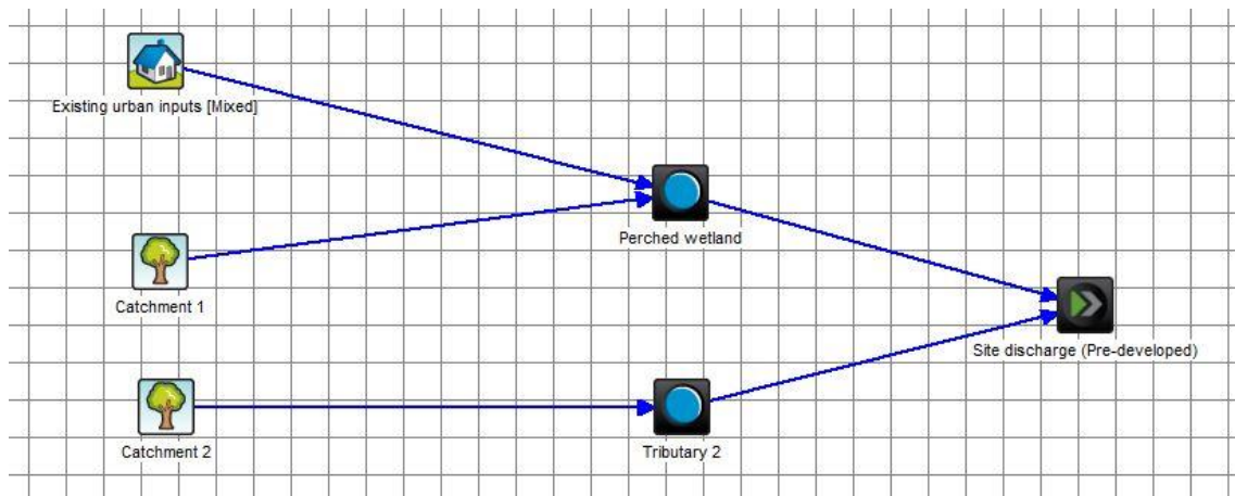
Figure 2: MUSIC structure for the pre-development condition
