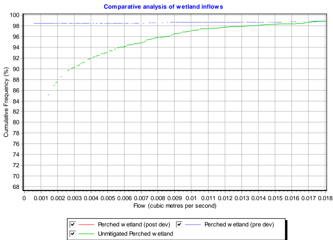
Figure 5: Cumulative frequency plot of discharge to perched wetland
