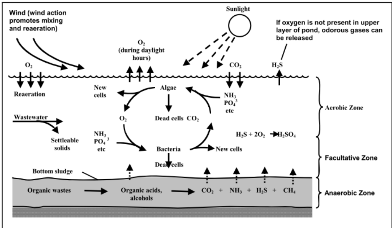
Figure 1: Treatment Processes in WSP's (Altner, 2005)
