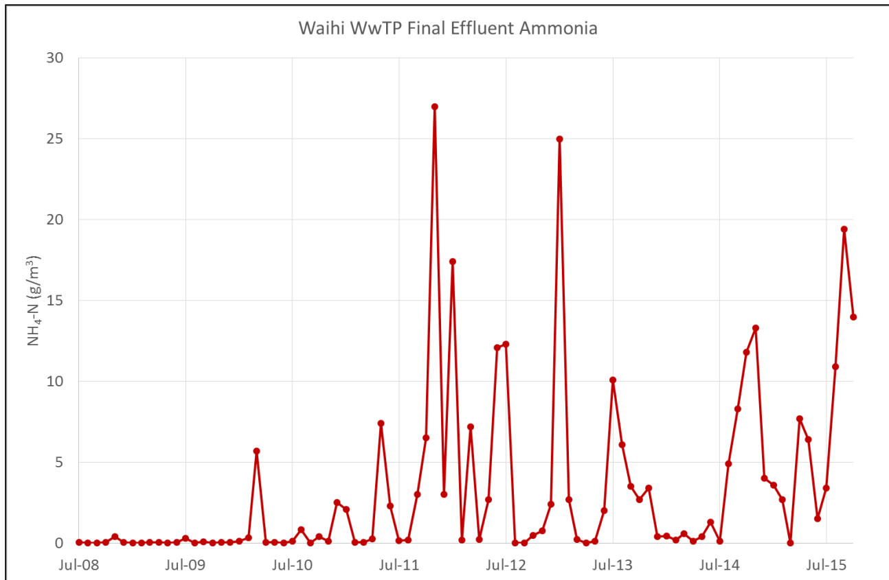
Figure 4: Effluent Ammoniacal Nitrogen at Waihi WwTP
