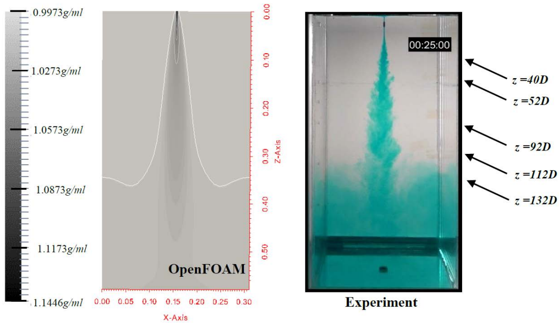
Figure 4 - Experimental observation and CFD prediction of a dense sugar jet ( Q = 4.1 \text{ ml/s} ) in a confined tank at t = 25\text{s} , showing the turbulent jet and the built up of dense fluid at the bottom
