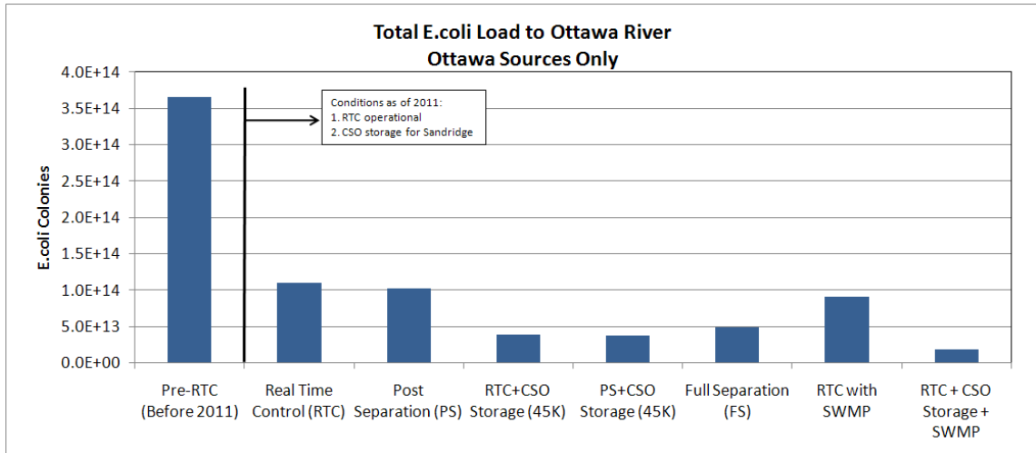
Figure 5 - Estimated E.coli load to the Ottawa River
