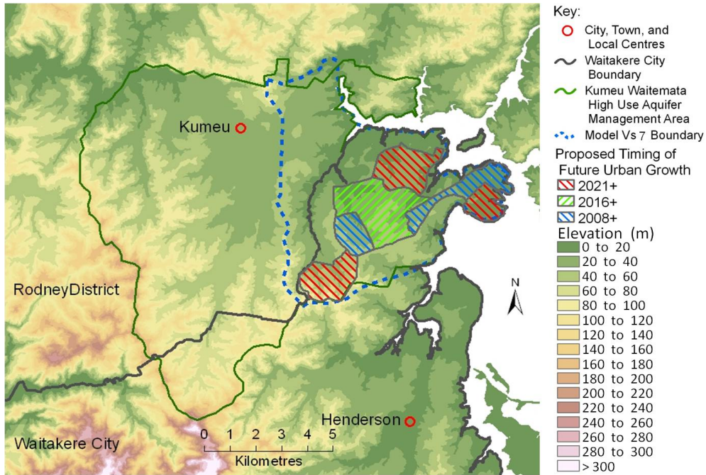
Figure 7: Topography of the NorSGA
