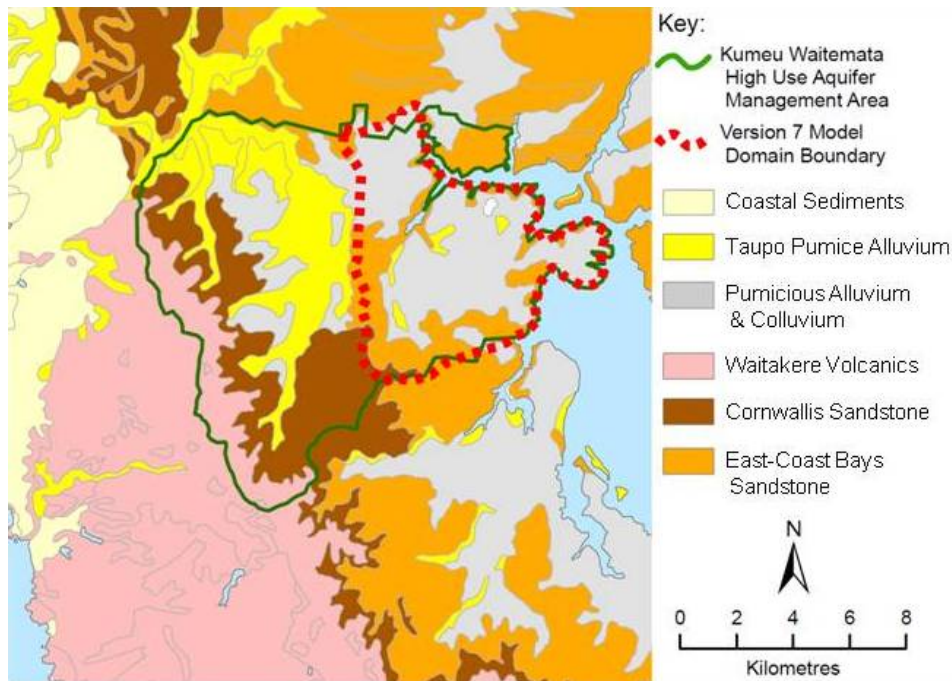
Figure 4: Simplified Geology of the NorSGA Area
