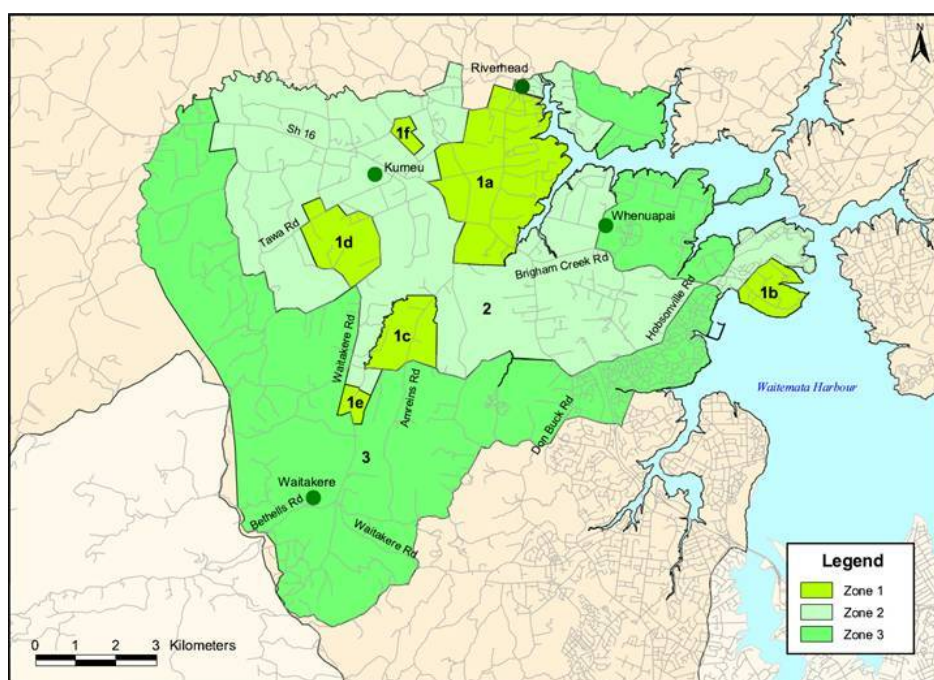
Figure 3: High Use Aquifer Management Area (ARC, 2001)
