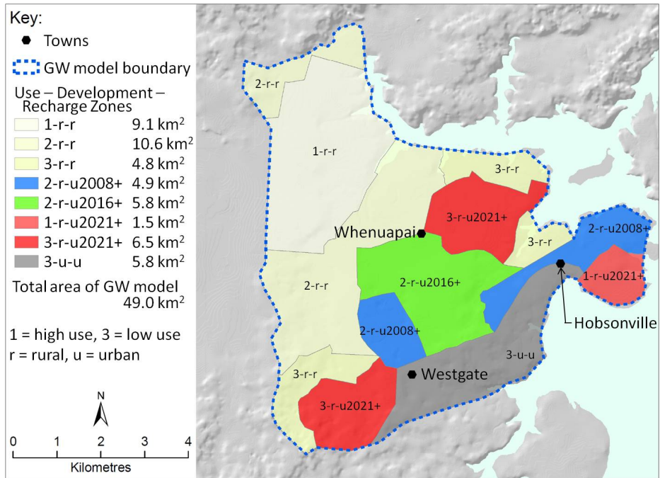
Figure 13: Ground-Water Use – Development – Recharge Zones
