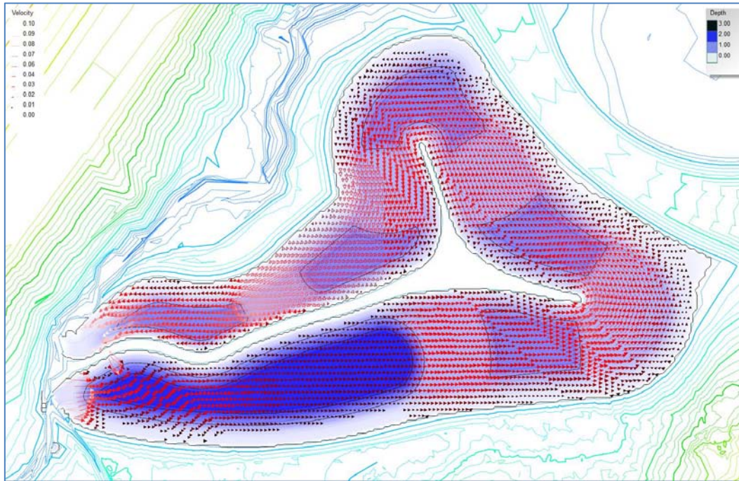
Figure 12: Steady State Simulation 0.5m 3 /s
