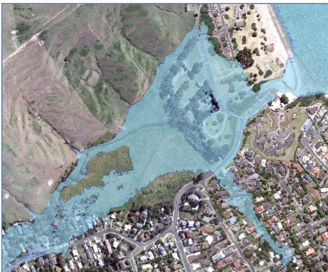
Figure 7: 100 Year Flood Extent Exclusive 2d Model
